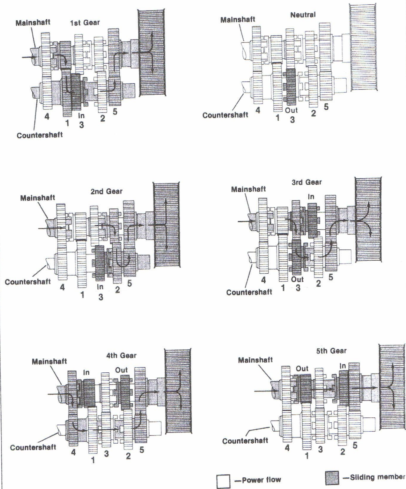
Figure 6-14. Transmission Power Flow
